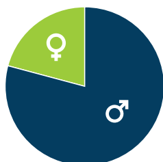
Figure 2: World cancer cases accountable to HPV. Adapted from [4].
