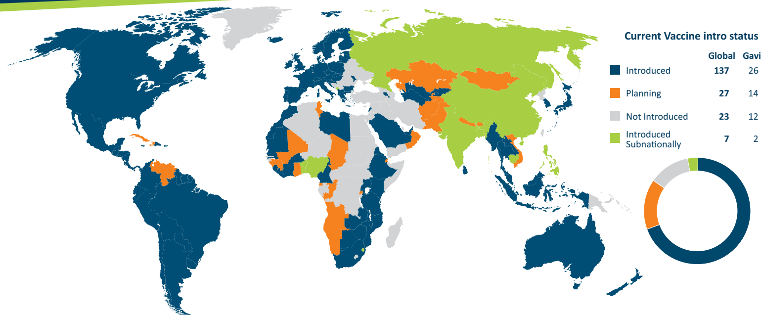
Figure 4: World map for HPV vaccines introduction into national immunization program. Adapted from [17].
