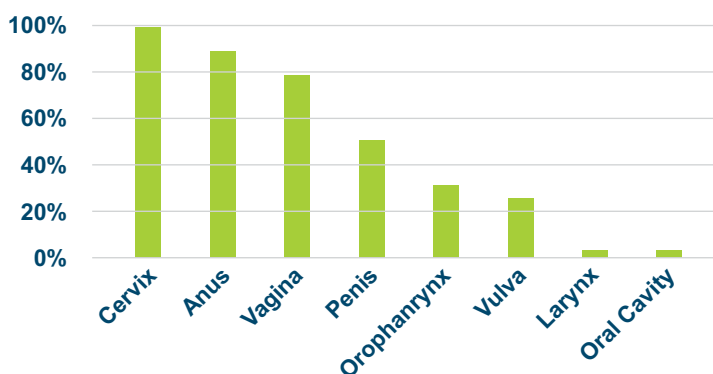
Figure 1: Frequency (%) of anogenital- and oropharyngeal cancers caused by HPV infection. Adapted from [4].
