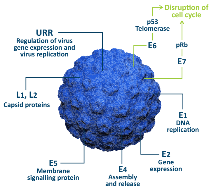
Figure 3: The HPV genome
